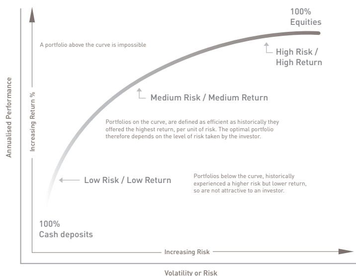
Figure 4: The efficient frontier
